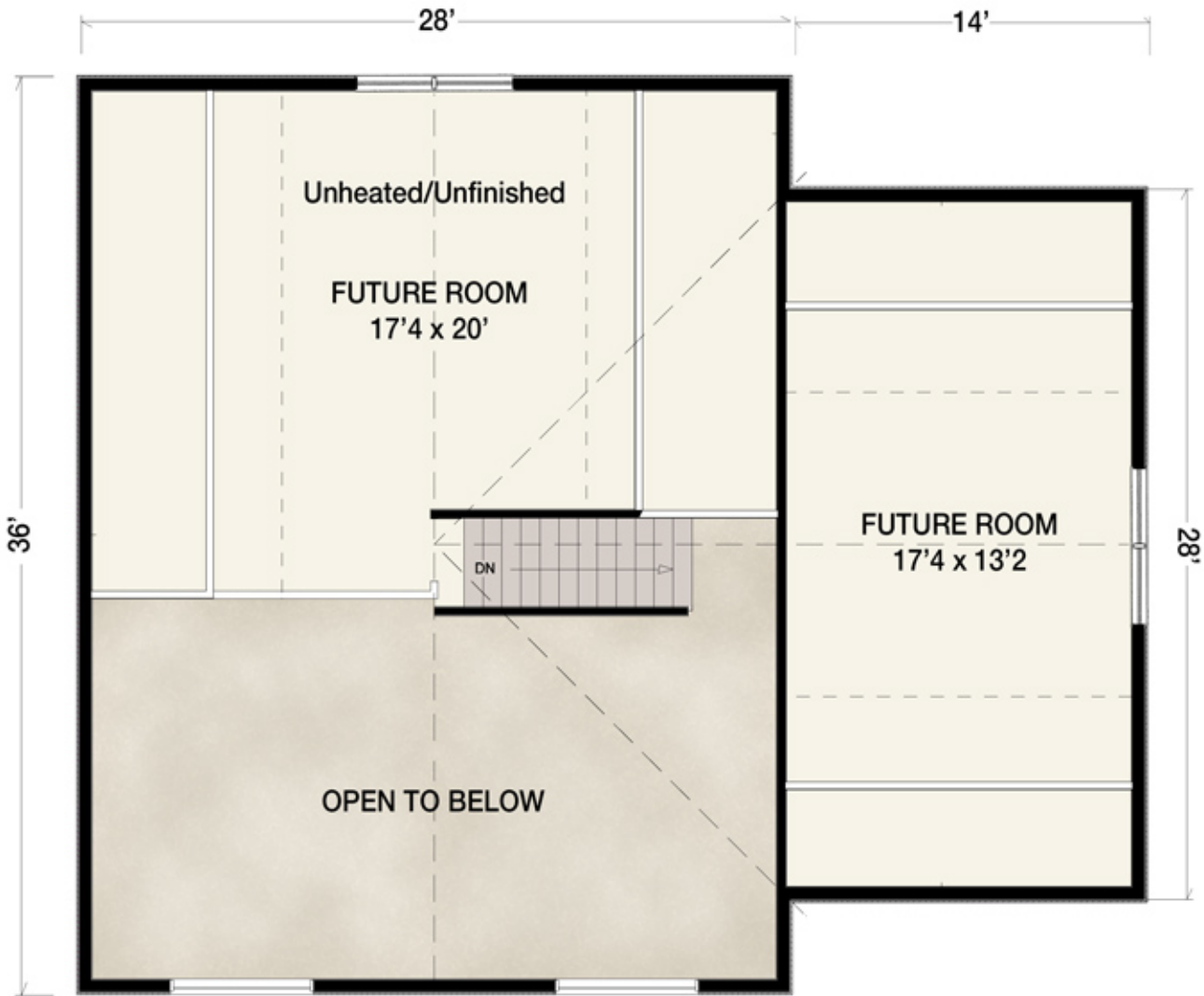
EAST SLOPE SECOND FLOOR
